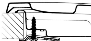
Hook position for H=40mm top
