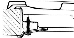
Hook position for H=20mm top
