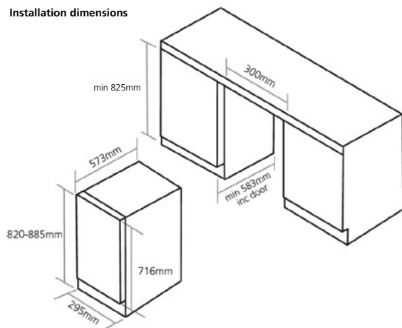
Installation dimensions
